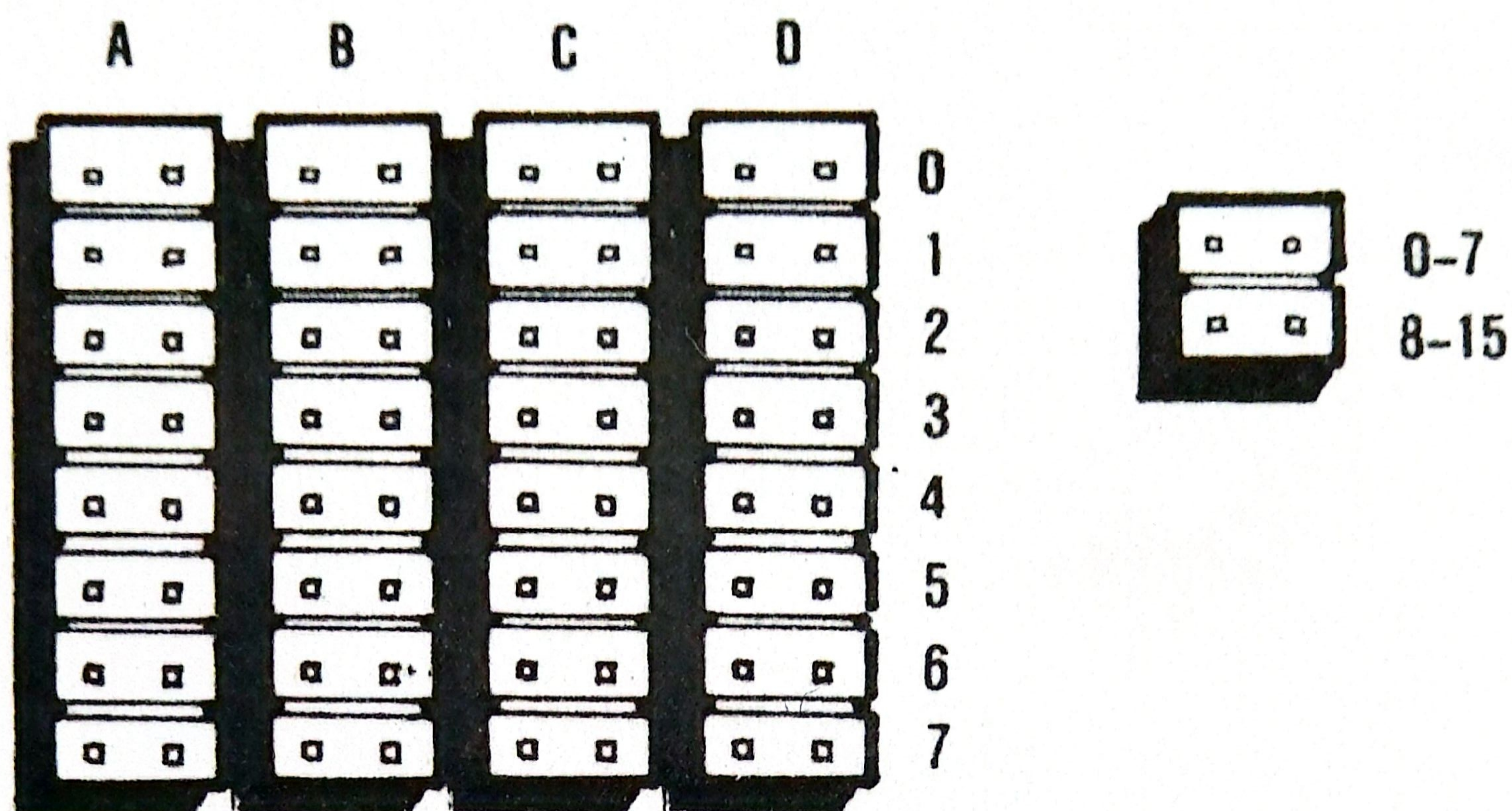
2-1: HS-RX1 ROM Expansion Card Layout
