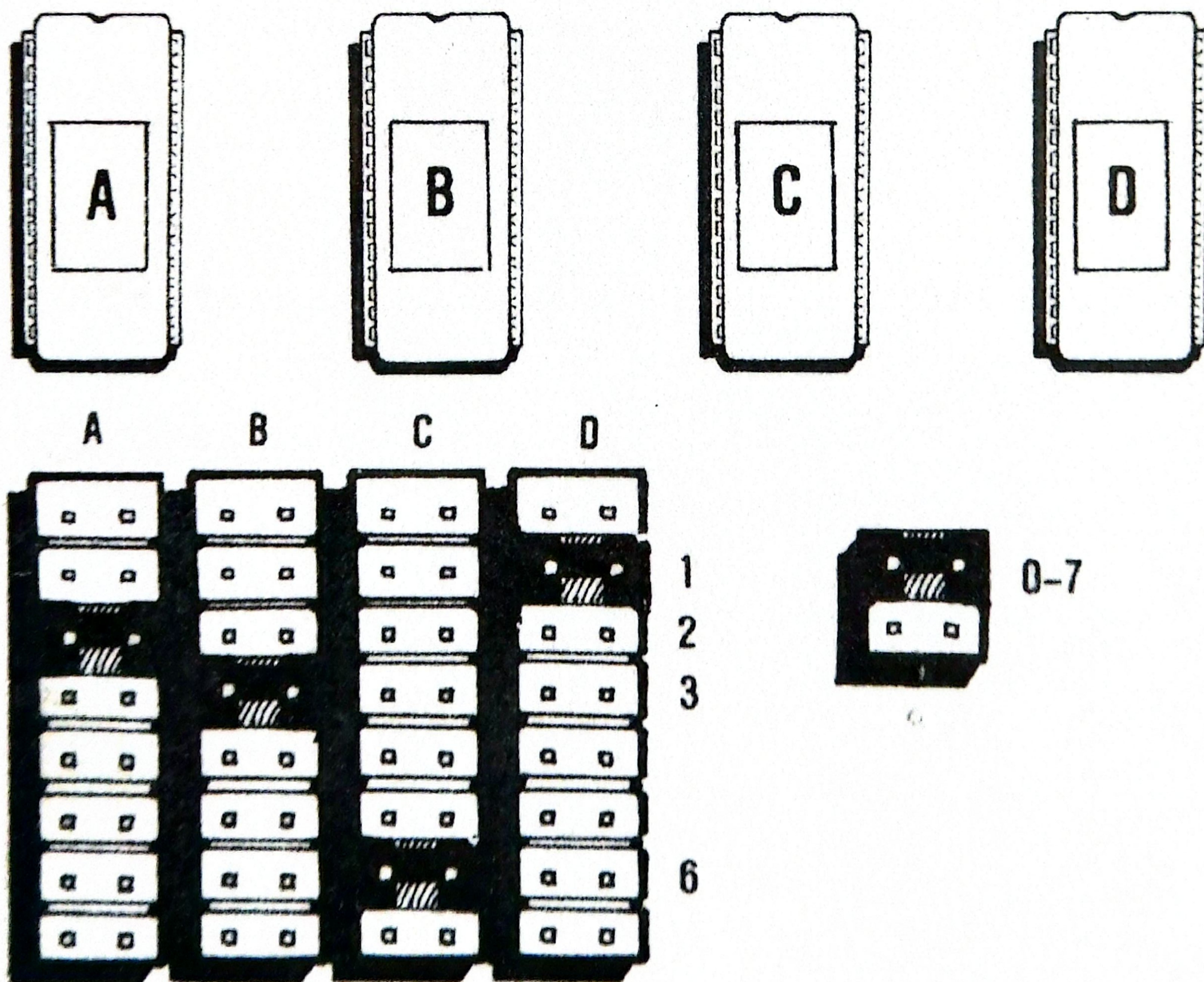
2-3: Example ROM Addressing
